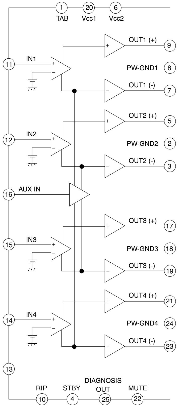
2. Block diagram
